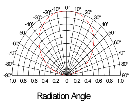
Radiation Characteristics
