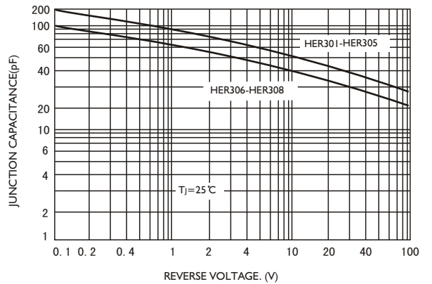
FIG.6-TYPICAL JUNCTION CAPACITANCE
