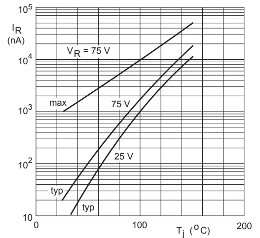
Fig.5 Reverse current as a function of junction temperature.
