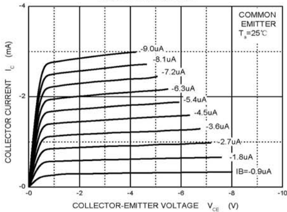
Static Characteristic
